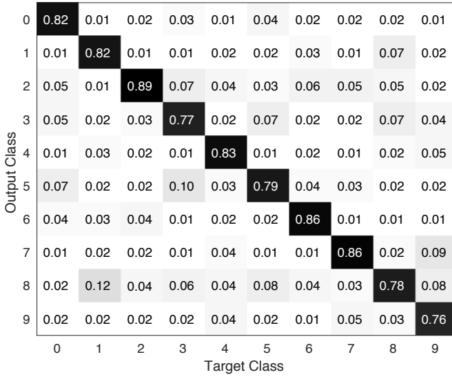
Fig. 6. Confusion matrix plot
