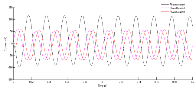
Fig. 10 Fault phase current waveforms
