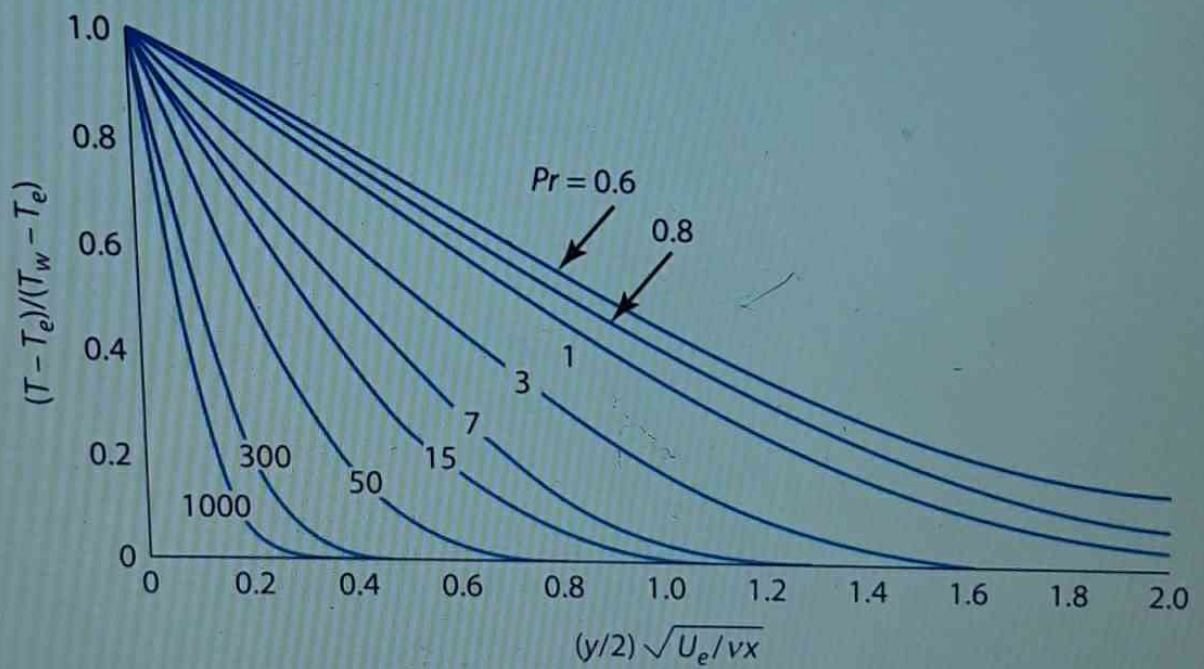
Fig. 4.5 Temperature profiles for laminar flow over a constant-temperature flat plate; from Eckert and Drewitz (1940).
