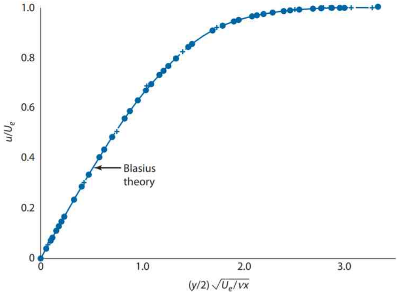
Fig. 4.3 Comparison between Blasius solution and experiments of Nikuradse for laminar flow over a flat plate; from Nikuradse (1942).
