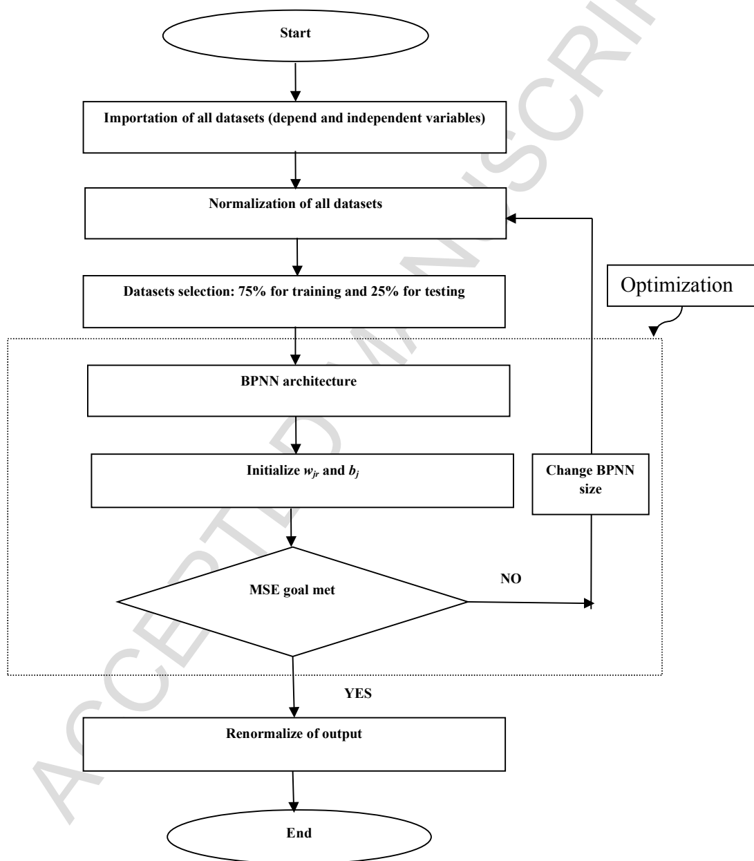
Fig. 2. The flow chart applied in the training of BPNN model.
