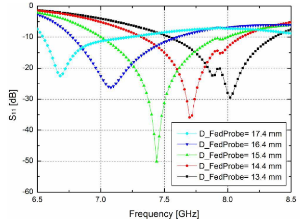
Fig. 3. Simulated reflection coefficient S_{11} for different diameters D\_FedProbe of the ring probe.
