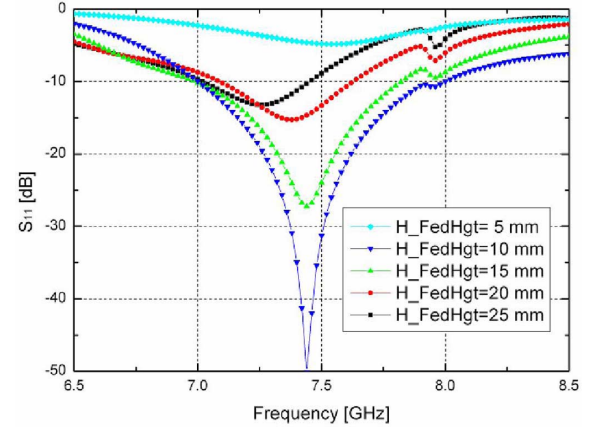
Fig. 2. Simulated reflection coefficient S_{11} for different vertical heights H\_FedHgt of the ring probe.
