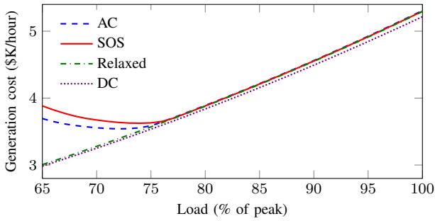
Fig. 2. Generation costs as a function of load for the 9-bus network.
