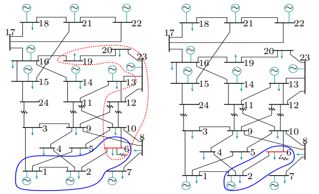
Fig. 3. IEEE 24-bus RTS with bus 6 isolated. On the left, DC method (solid) and PWL method without shunt switching (dashed). On the right, PWL method with shunt switching.
