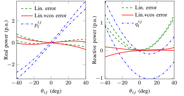
Fig. 1. Maxima and minima of power flows, and of approximation errors, as a function of phase angle difference.
