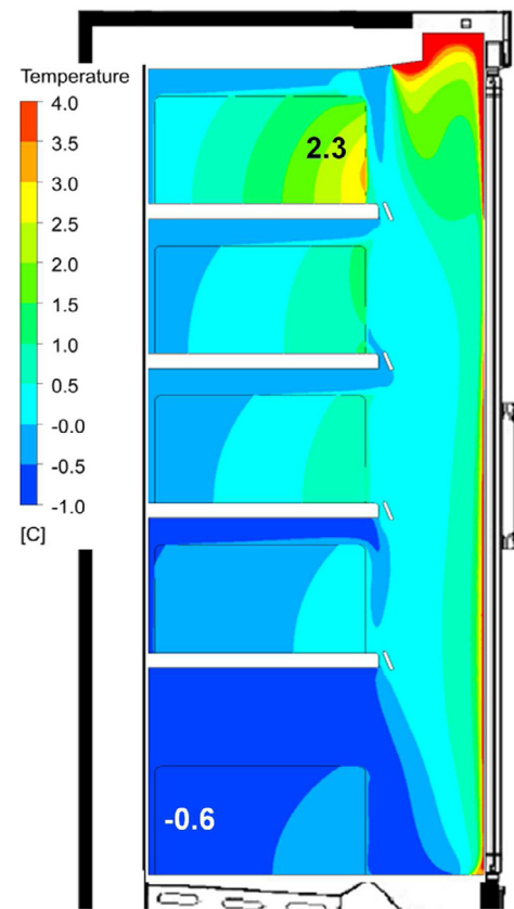
Fig. 7. Numerical prediction of the internal temperature distribution in a closed display cabinet. (For interpretation of the references to colour in this figure legend, the reader is referred to the web version of this article.)
