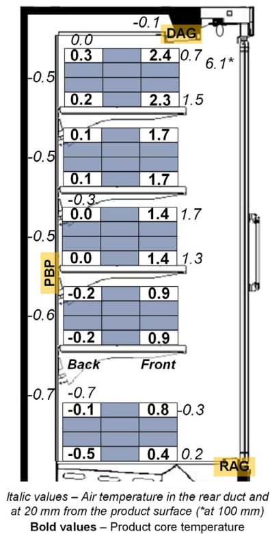
Fig. 3. Experimental result of air and product temperature distributions in a closed display cabinet (Chaomuang et al., 2019a).
