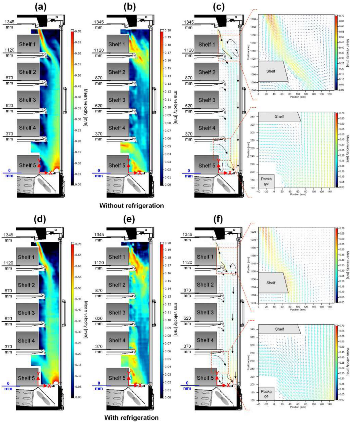
Fig. 2. Mean air velocity profiles (a); velocity fluctuations (b); and velocity vector fields (c); along the air curtain of a closed display cabinet running with fans only (refrigeration system “off”). Mean air velocity profiles (d); velocity fluctuations (e); and velocity vector fields (f); along the air curtain of a closed display cabinet running with fans and the refrigeration system “on”.
