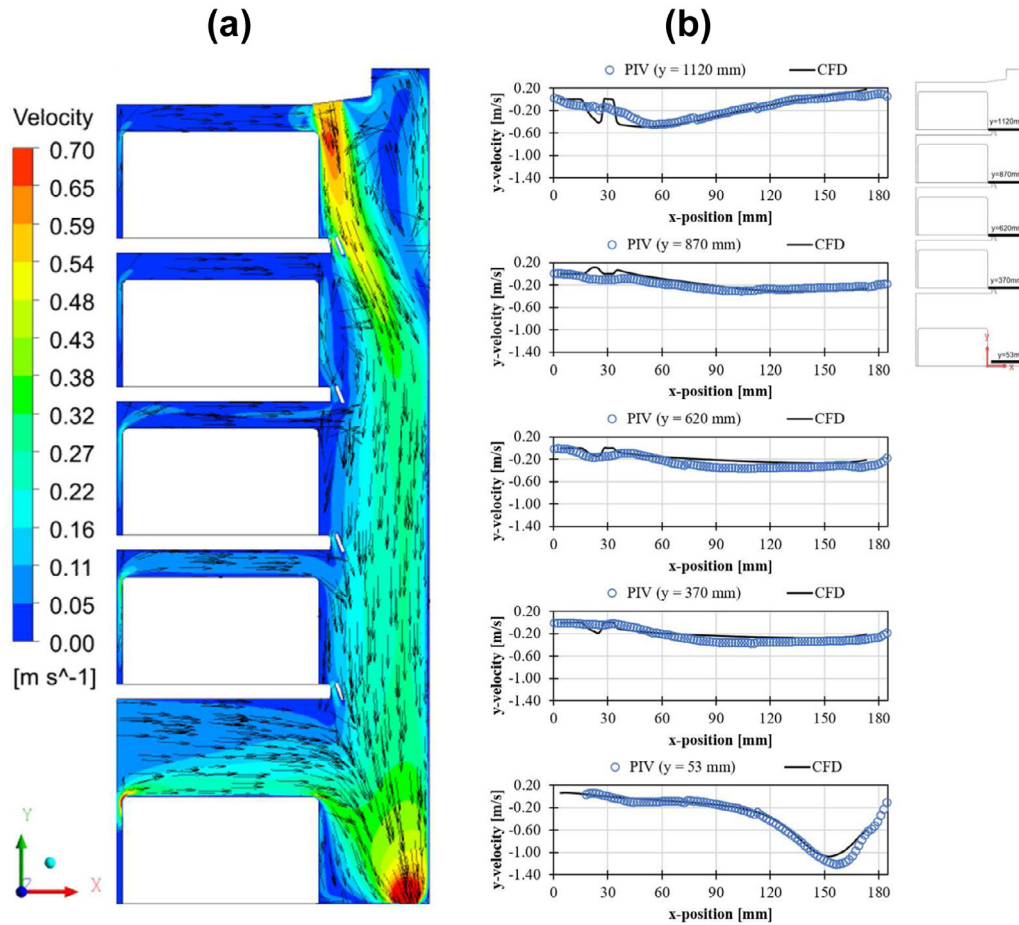
Fig. 6. (a) Predicted air velocity profile in a closed refrigerated display cabinet (b) comparison between experimental (PIV) and numerical (CFD) results. (For interpretation of the references to colour in this figure legend, the reader is referred to the web version of this article.)
