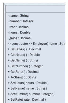
UML class diagram
