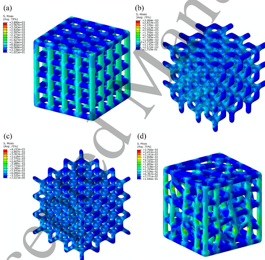
Figure 13. Von-Mises contour plots for different porous scaffolds with 70% porosity. (a) Cube scaffolds. (b) Diamond scaffolds. (c) Rhombic dodecahedron scaffolds. (d) Irregular porous scaffolds.
