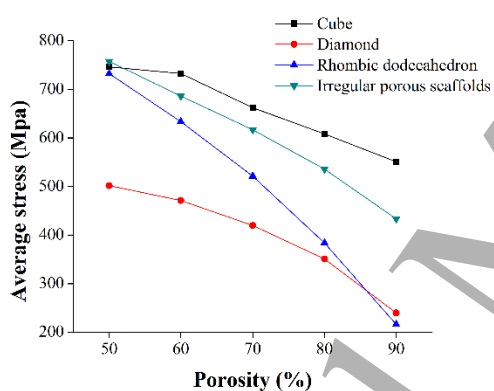
27 28 29 30 31 32 33 34 35 36 37 38 39 40 Figure 11. Relation between porosity and average stress of four porous scaffolds.
