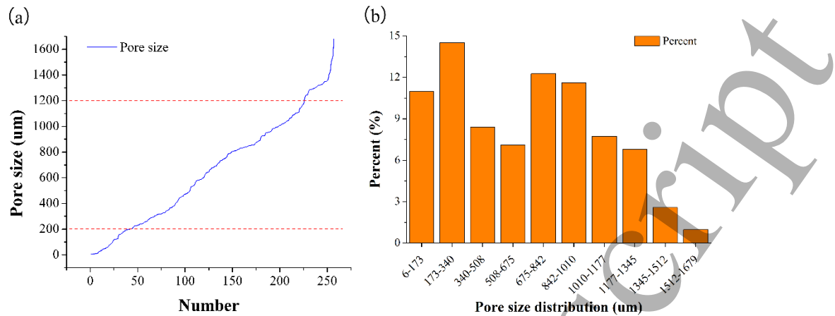
Figure 5. Pore size distribution of irregular porous scaffold with porosity of 70%. (a) Curve graph.
