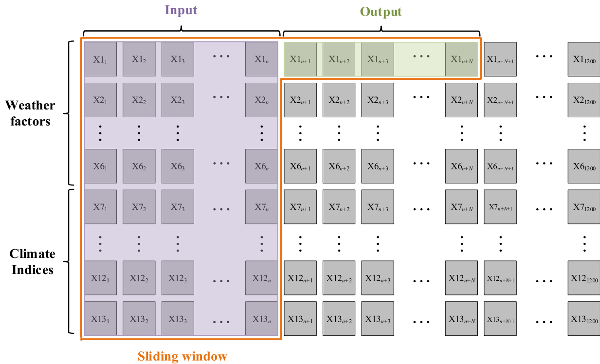
Fig. 6. Sample generation using a sliding window.
